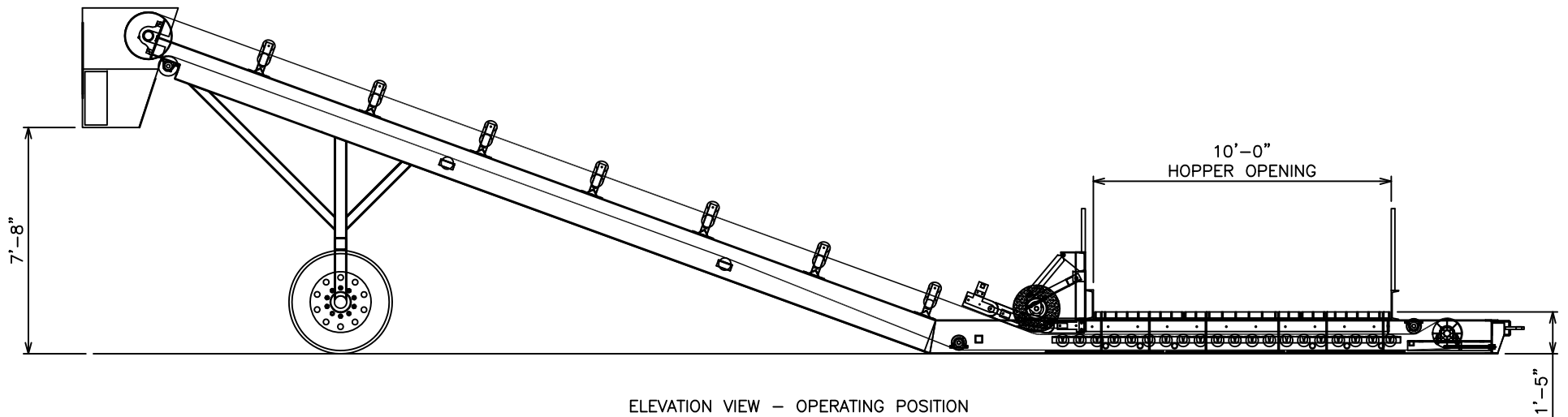
ELEVATION VIEW – OPERATING POSITION
